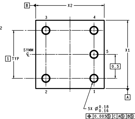
5-Bump micro SMD Ball Grid Array Package Order Number LM74CIBP-3, LM74CIBPX-3, LM74CIBP-5, LM74CIBPX-5 NS Package Number BPD05MPB The following dimensions apply to the BPD05MPB package shown above: X1=1565µm ±30µm, X2=1615µm ±30µm, X3=850µm ±50µm.
